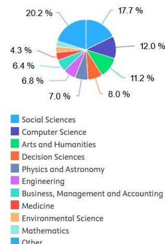
Subject trends
